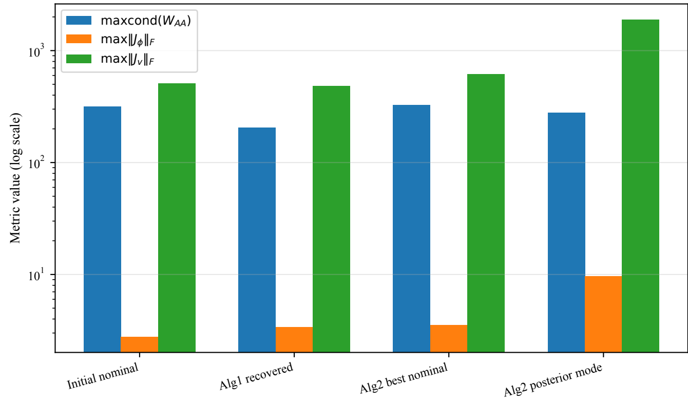
Batch linearization stability metrics
